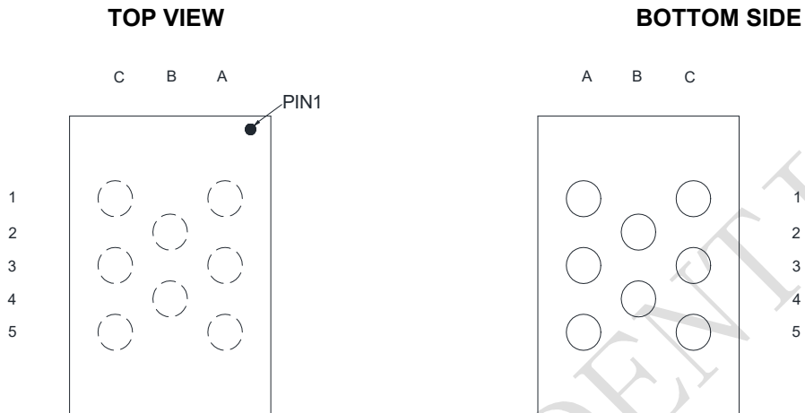
Figure 1-1 WLCSP8 Pin Configuration
